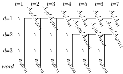
Figure 2: Mapping of schematized right-corner tree into HHMM memory elements.
