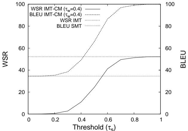
Figure 2: BLEU translation scores versus WSR for different values of the sentence classification threshold using the RATIO CM with \tau_w = 0.4 .
